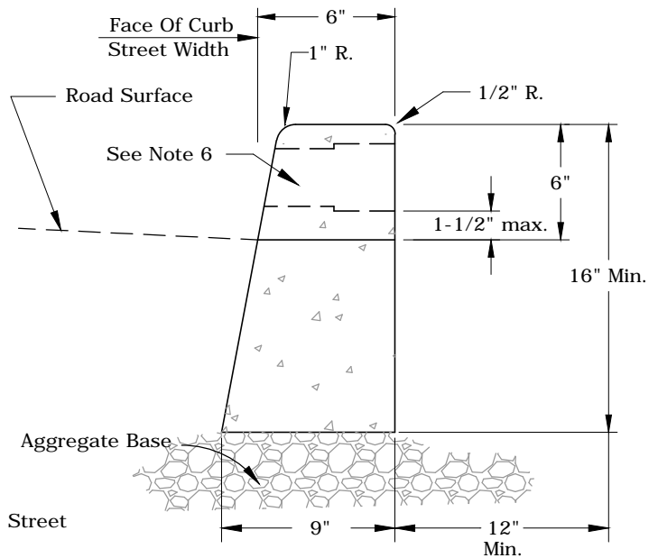
VERTICAL CURB DETAIL
