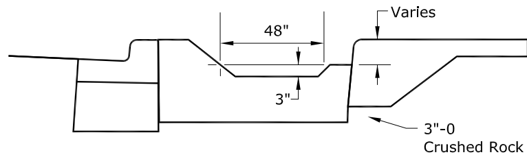
ROCK CHECK DAM DETAIL
