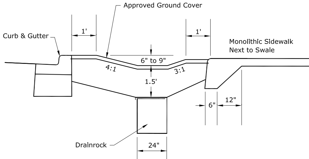
RAIN GARDEN TYPICAL SECTION
