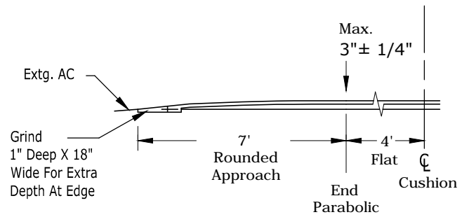
SECTION VIEW A - A Symmetrical About C N.T.S.
