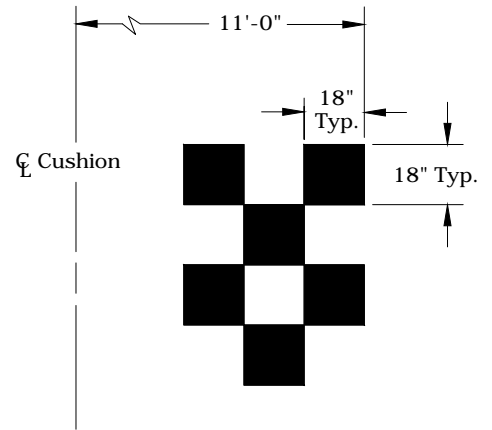
PAVEMENT MARKING DETAIL N.T.S.
