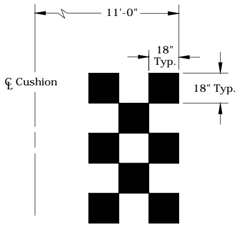
PAVEMENT MARKING DETAIL N.T.S.
