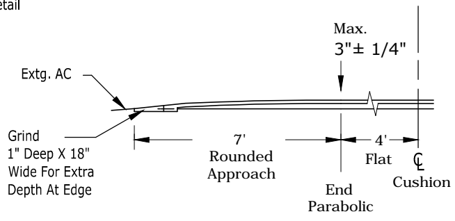
SECTION VIEW A - A Symetrical About ☒ N.T.S.
