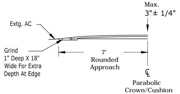
SECTION VIEW A - A Symmetrical About CL N.T.S.
