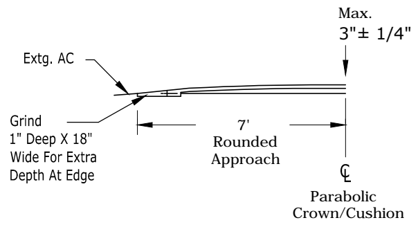
SECTION VIEW A - A Symmetrical About \bar{C} N.T.S.
