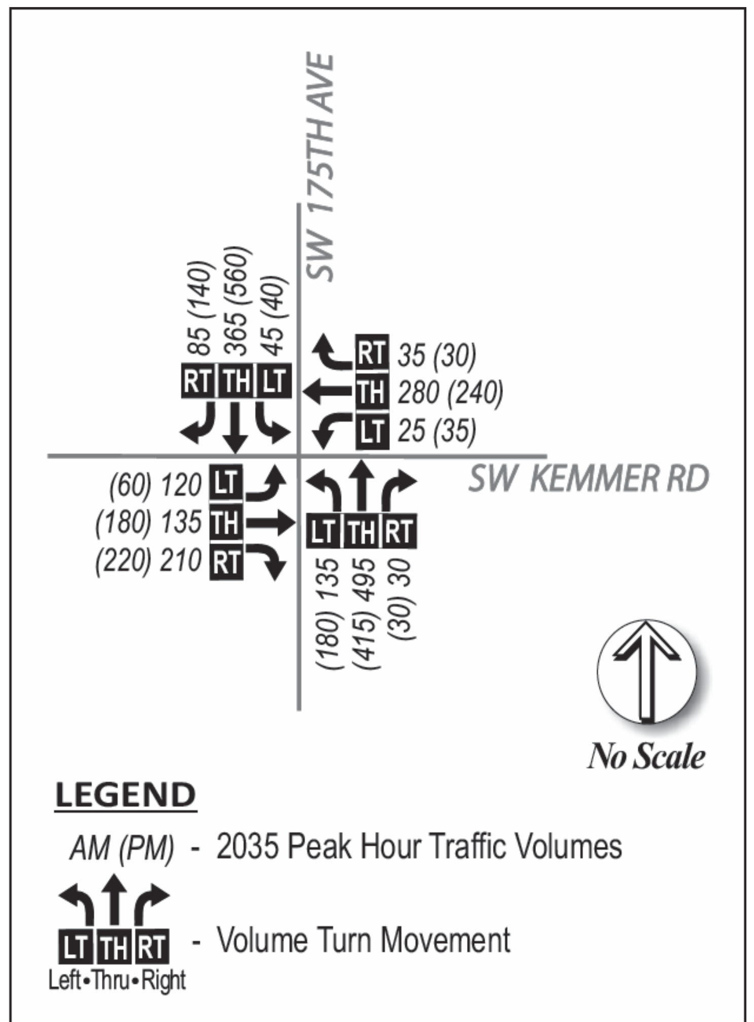
DESIGN YEAR PROJECTION (2035)
